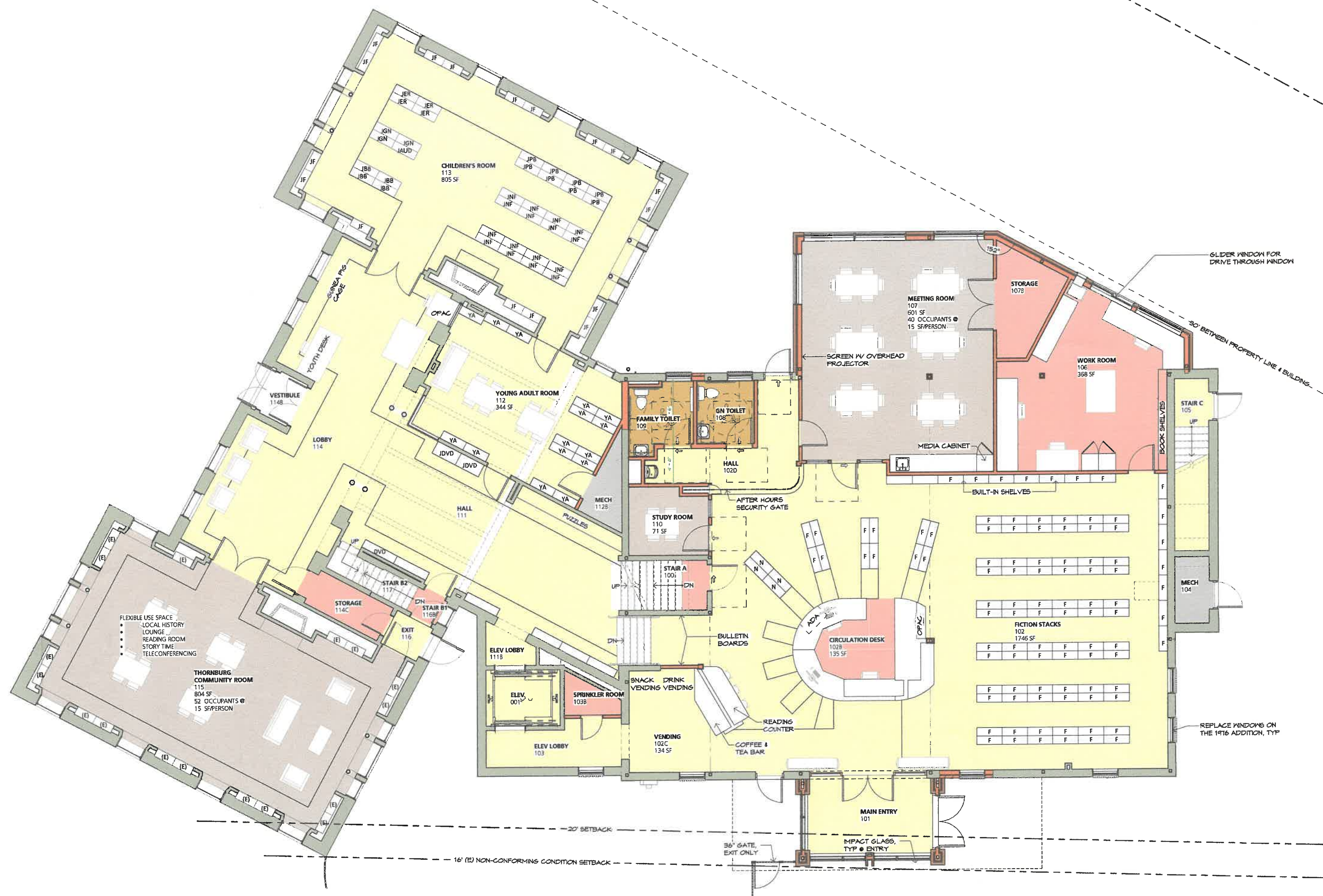
1 PROPOSED FIRST FLOOR AND MAIN FLOOR LEVELS - PRESENTATION 8101 3/16" = 1'-0"
